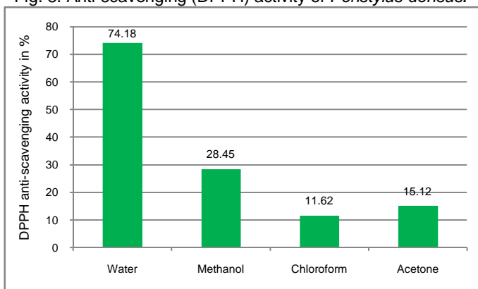
Fig. 8. Anti-scavenging (DPPH) activity of Peristylus densus .
