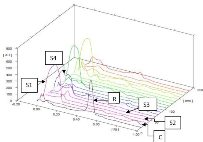
Fig. 11. HPTLC peaks of standard and tuber extracts of P. densus .
