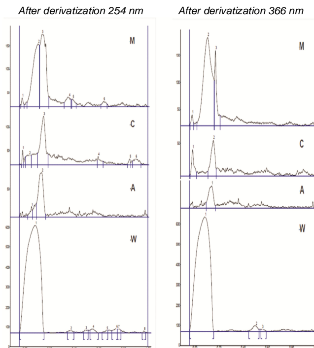
Fig. 10. HPTLC peaks at 254 nm and 366 nm after derivatization of tuber extracts of P. densus .
