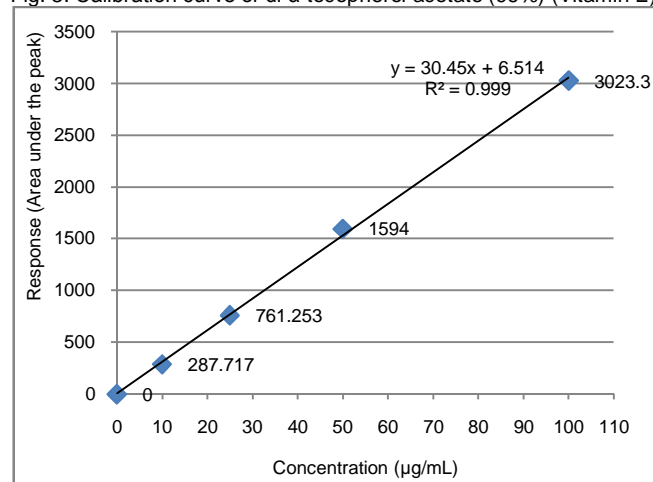
Fig. 3. Calibration curve of dl α-tocopherol acetate (96%) (Vitamin E).
