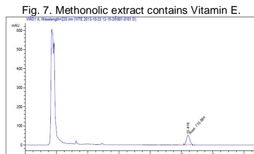
Fig. 7. Methonolic extract contains Vitamin E.
