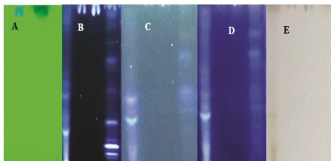
Fig. 9. HPTLC-Chemical profiling of flavonoids in tuber extracts of Peristylus densus .
